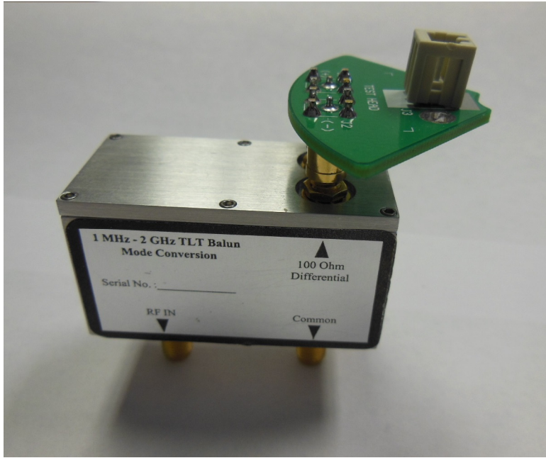
TLT 2.0 GHz Balun
